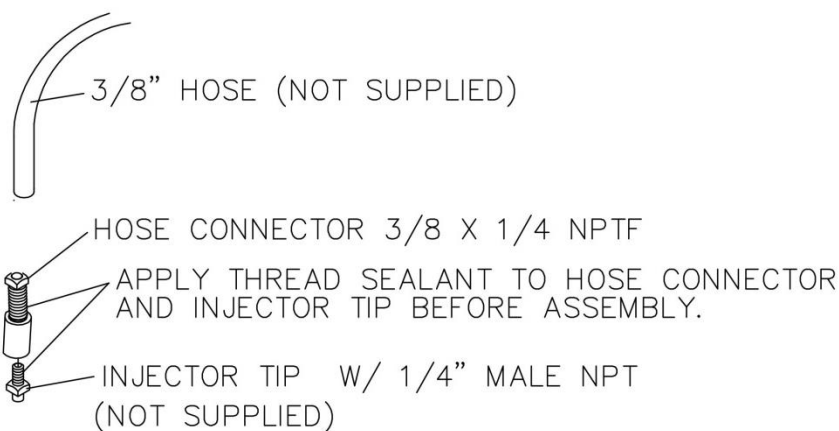
ISO-2968-020A-INJECTOR PLUMBING
